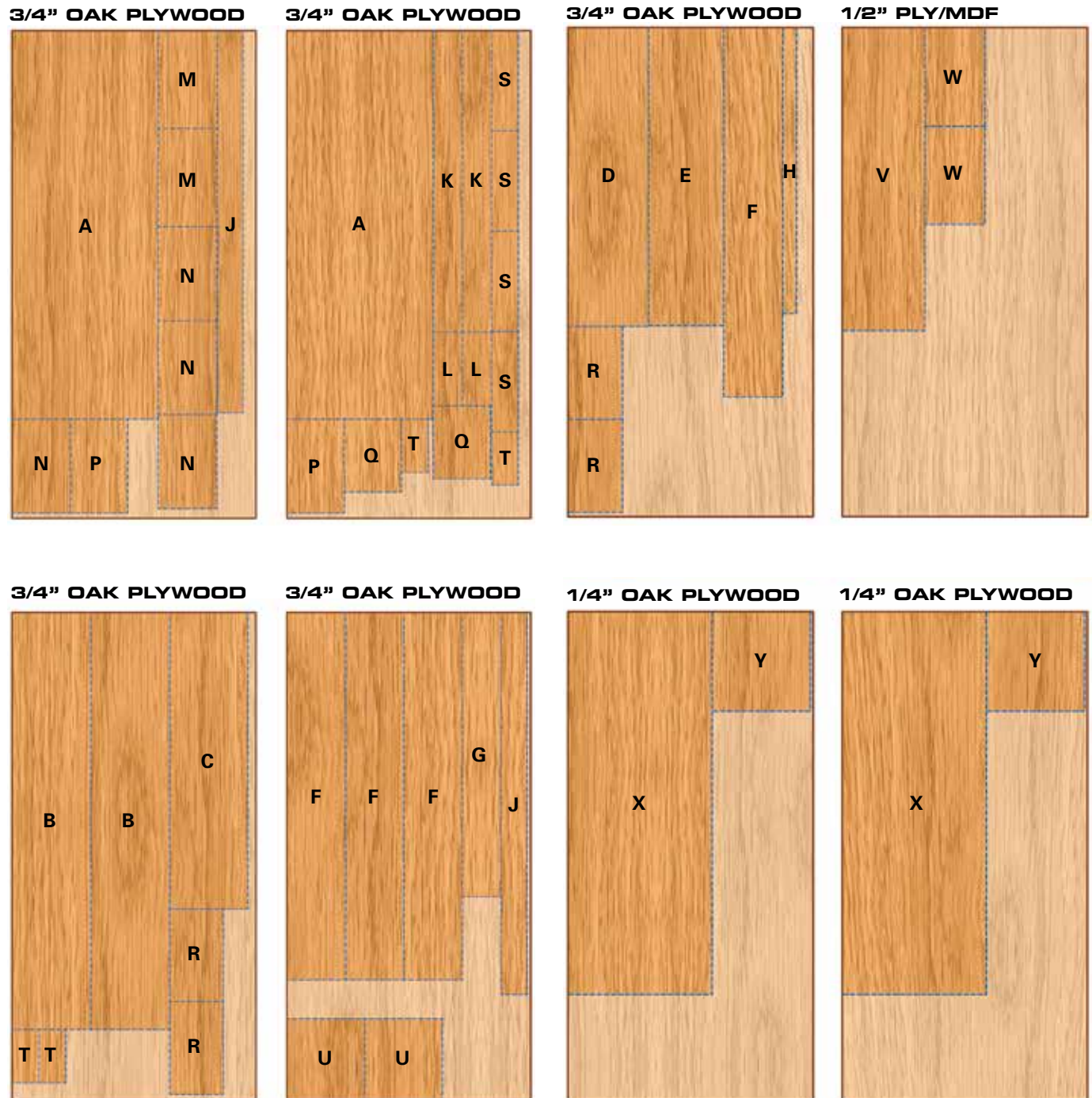
Figure D Plywood cutting diagrams
