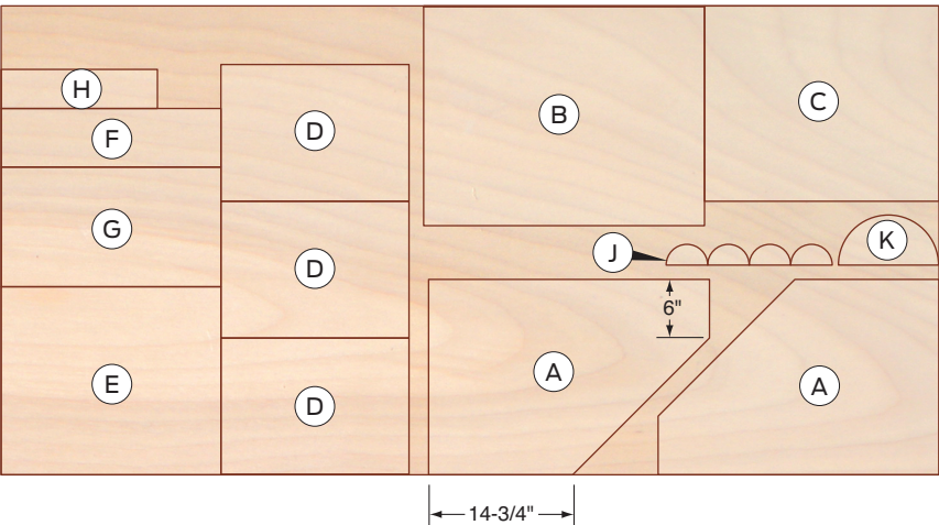
Figure B Plywood cutting diagram
